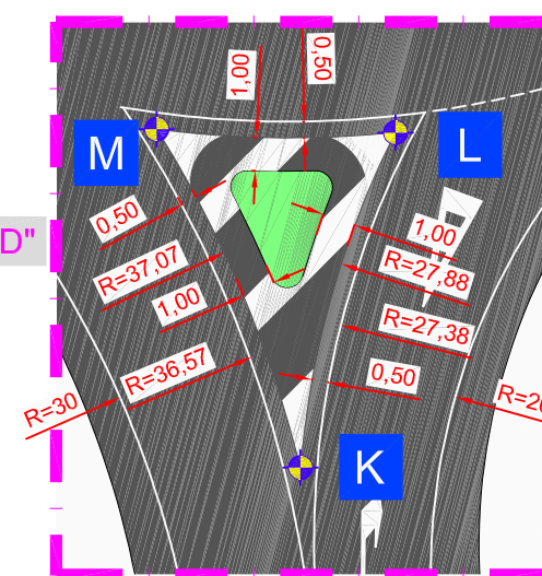
DETALLE "D"
